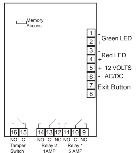
Layout of connector blocks on CA5
